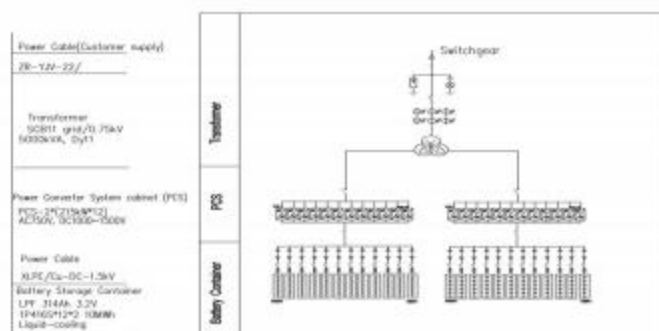
5MW/10MWh BESS Single-line Diagram
